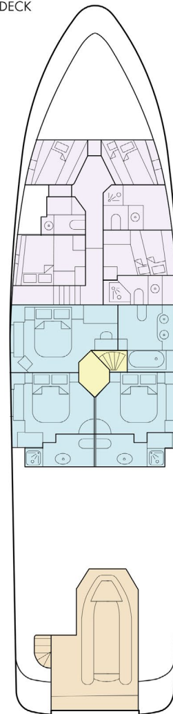
LOWER DECK
